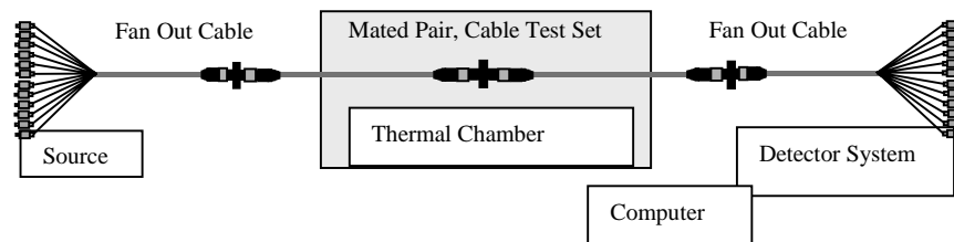
Figure 6: Thermal cycling experimental test set up.
