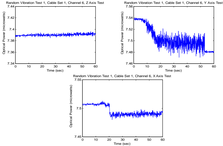
Figure 3: Random vibration data during z, y, and x axis tests of cable set 1, channel #6
