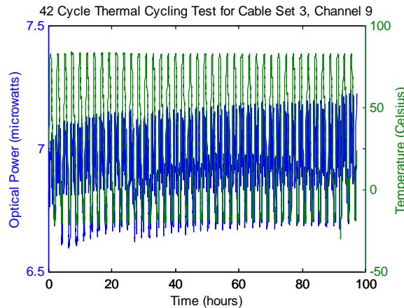
Figure 9: Thermal cycling 42 cycles from -20^{\circ}\text{C} to +85^{\circ}\text{C} , 3^{\circ}\text{C}/\text{min} up, 2^{\circ}\text{C}/\text{min} down, optical power on left axis, temperature on right axis for cable set 3
